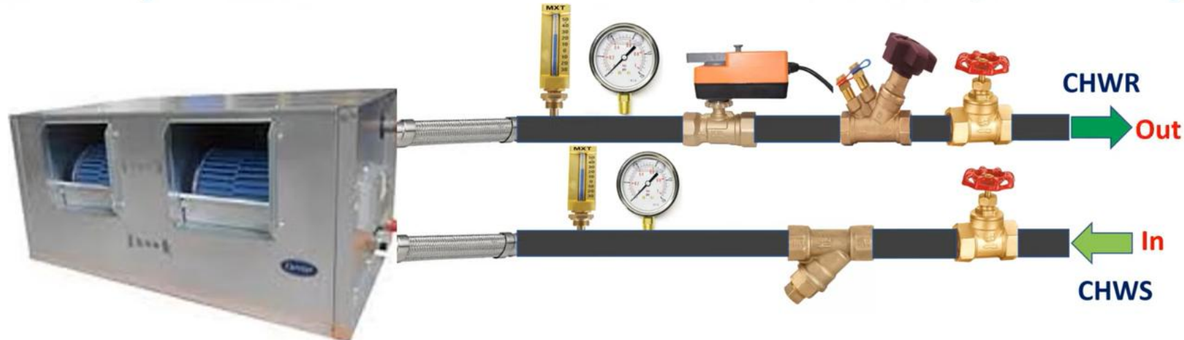
Balancing Valve
